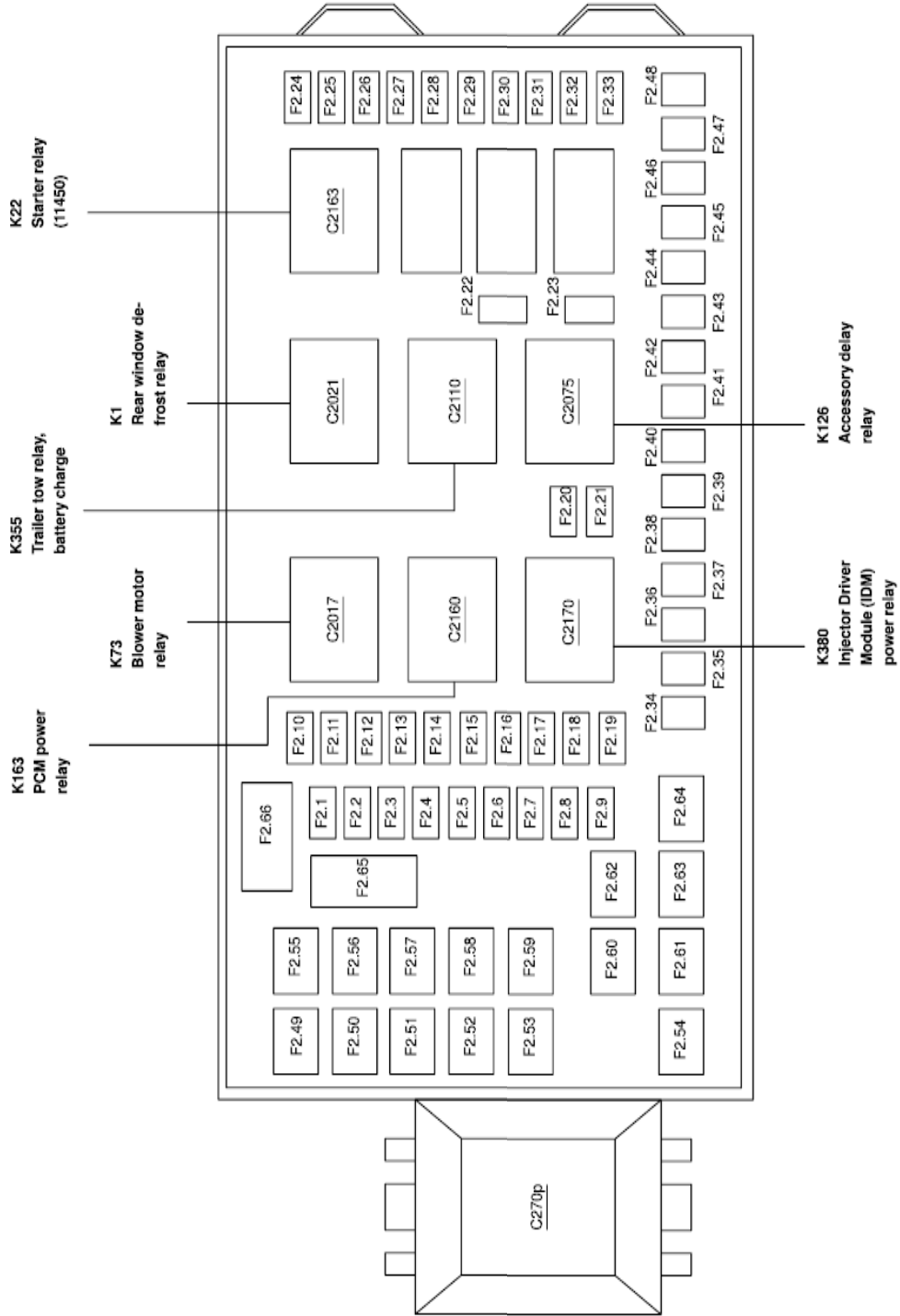
Central Junction Box (CJB) (14A068)
